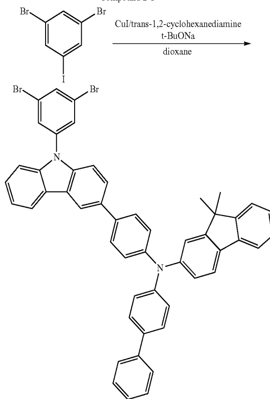
Compound 2
