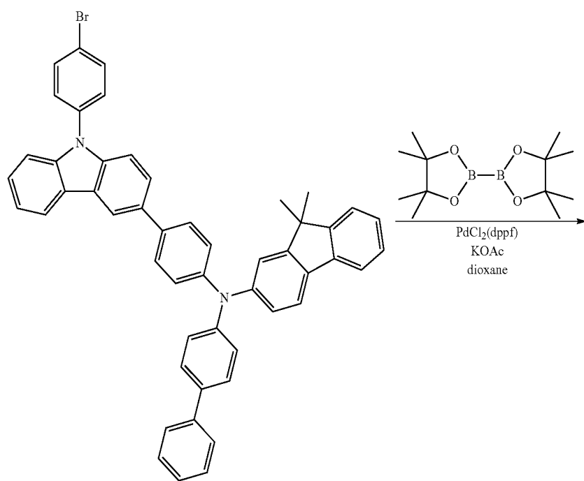
Compound 5-1
