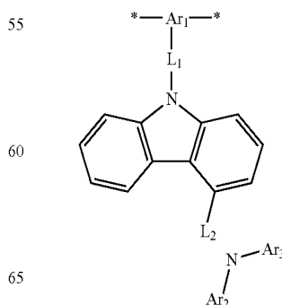
Chemical Formula 1
