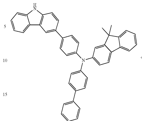
Compound 2-1
