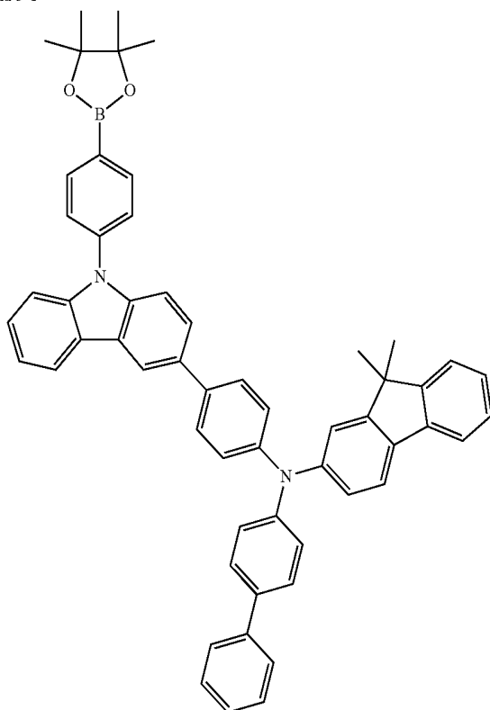
Compound 5-2
