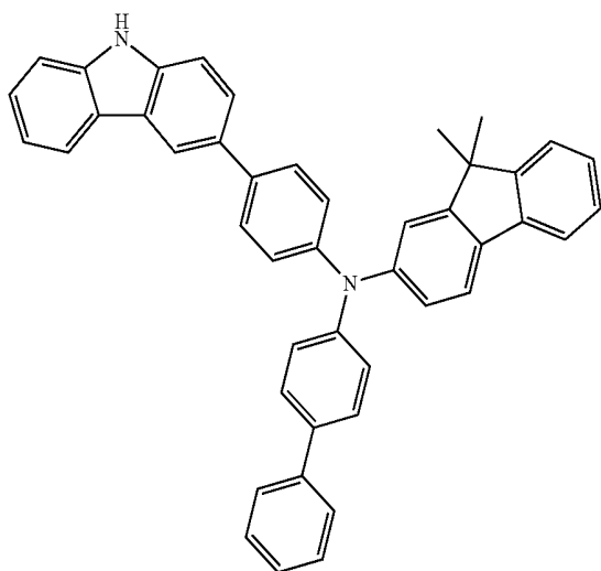
Compound 2-1
